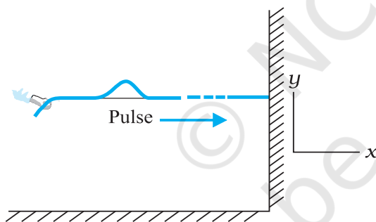
Fig. 14.2 When a pulse travels along the length of a stretched string ( x -direction), the elements of the string oscillate up and down ( y -direction)
